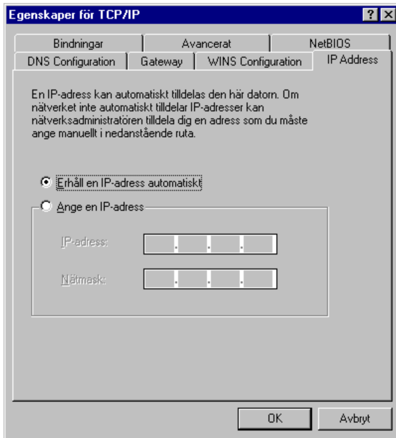
Figur 7, Windows 95 DHCP-klient
