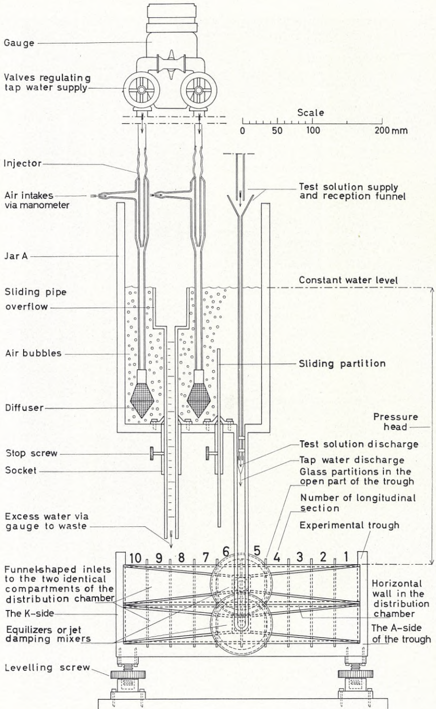
Fig. 3. Scheme of the fluvium as seen from its upstream end.
