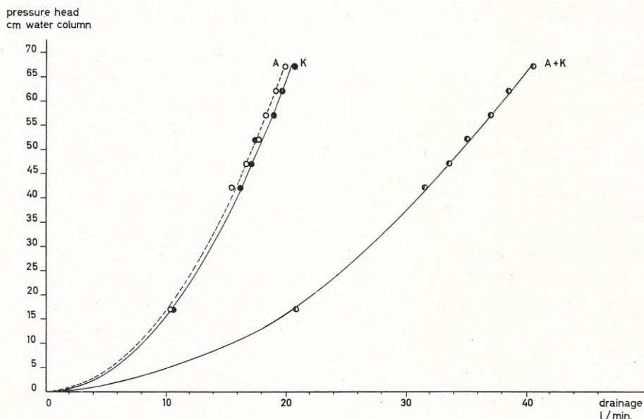
Fig. 4. Pressure head in the fore-jars in relation to drainage through the experimental flume. A and K denote the flow from the respective fore-jars; A+K the total one.
