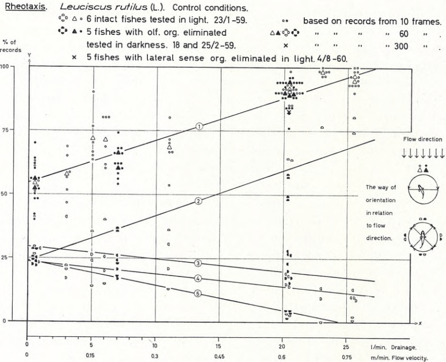
Fig. 20. Rheotactic orientation of roach in relation to flow velocity through the test yard. Encircled figures signify the centre coordinates of regression lines the equations of which are given in Table 11.
