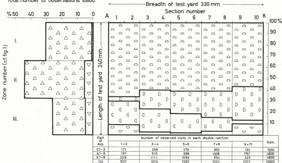
Fig. 22. The way or rheotactic orientation in various double sections and zones of the test yard (cf. Fig. 1). All records from the symmetrically arranged experiment of Dec. 18, 1958 (Fig. 11) are considered. For the explanation of the symbols see Fig. 20; cf. also p. 71.
