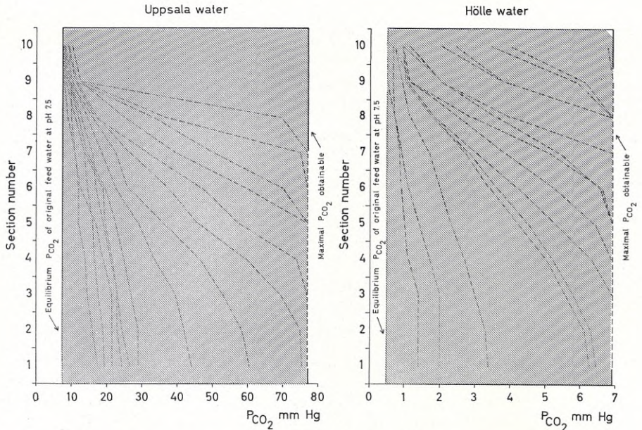
Fig. 35. Auxiliary graph for the construction of the reaction diagrams of Figs. 36 and 37. Considering different standard gradients of \alpha_1 -type established in Uppsala and Hölle water, the mean P_{CO_2} from all experiments at the same standard conditions are plotted against the section number of the test yard (Fig. 1). Cf. p. 99.
