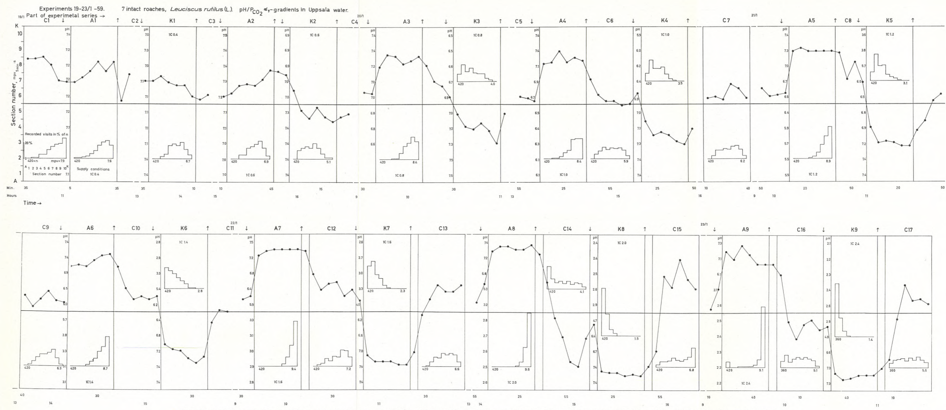
Fig. 12. Experimental diagram (cf. p. 49) showing the preference reactions of seven intact roaches in steeper and steeper \alpha_1 -gradients (A1-A9 and K1-K9) of combined pH/P CO2 in Uppsala water and during intervening control periods (C1-C17). Using the pH values measured in situ the corresponding P CO2 values can be taken from Fig. 6. Cf. also Figs. 29, 31, and 36.
