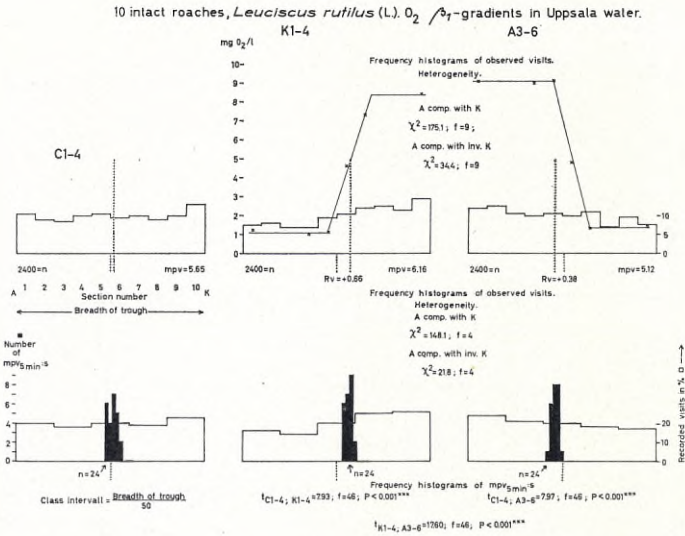
Fig. 25. Preferred sections (upper frequency histograms; cf. p. 46) and preferred double sections (lower ones) of roach in pure Uppsala water (C1—4) and in corresponding inverted \beta_1 -gradients of O 2 (lines and crosses at K1—4 and A3—6). Black areas show the distributions of mpv_{5min} . For the explanation of the statistics see the text on pp. 65. Cf. also Figs. 17 and 26.
