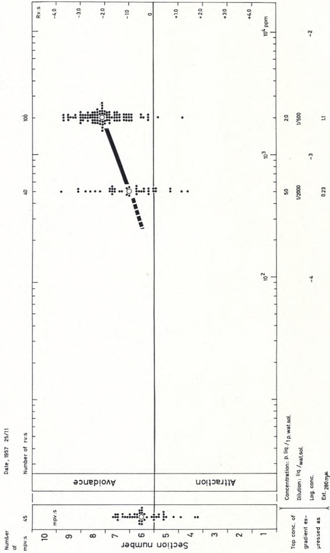
Fig. 48. Reaction diagram (cf. p. 56 and Fig. 42) based on the observational material also presented in Fig. 18.
