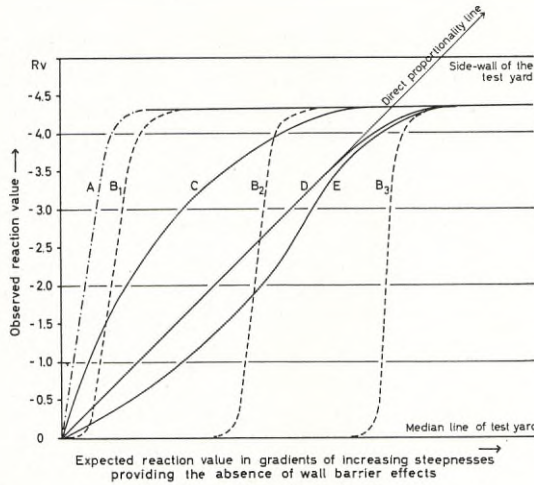
Fig. 24. Hypothetical scheme of the essential differences in the effects of the confined space which might be expected upon the observed rv on account of specifically diverse behaviour patterns. A, Species with stations in the open water and predilection for wall proximity, e.g. Gasterosteus aculeatus . B, Species with more ( B_2 and B_3 ; e.g. parr of Salmo salar and S. trutta ) and less ( B_1 ; e.g. parr of S. alpinus and S. fontinalis ) fixed stations on the bottom and a certain predilection for wall proximity. C, Free-moving species which prefer to stay near the lateral walls, e.g. young of Perca fluviatilis . D, Free-moving species which are more evenly recorded all over the width of the test yard, e.g. Leuciscus idbarus . E, Free-moving species which tend to avoid the lateral sections, e.g. Leuciscus rutilus .
