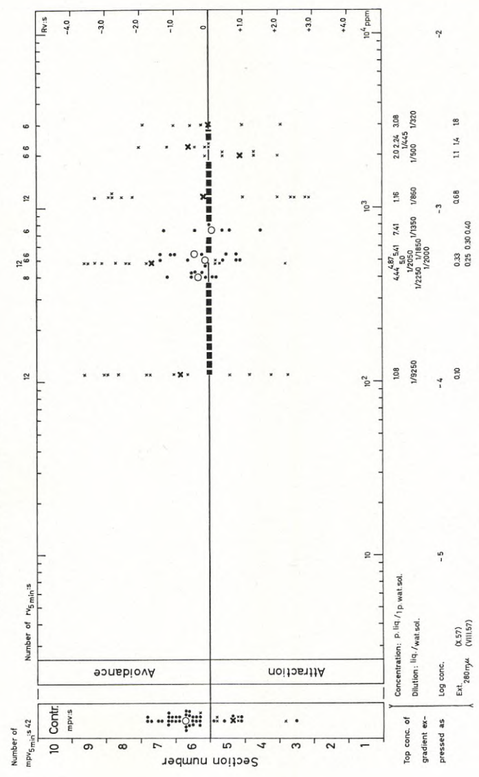
Fig. 49. Reaction diagram (cf. p. 56 and Fig. 42) showing the results of two experimental series performed with Coregonus nasus .
