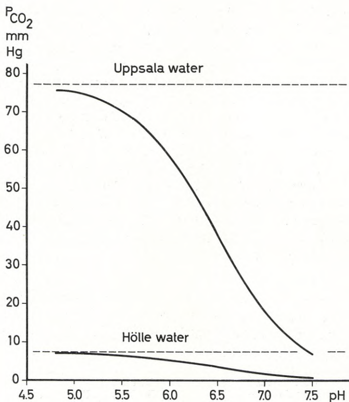
Fig. 6. The relationships between pH and P_{\text{CO}_2} calculated for the two kinds of feed-water according to expression (4) on p. 38. The maximum P_{\text{CO}_2} values which can be obtained by the acidification of Uppsala and Hölle water are demonstrated by horizontal lines of short dashes.
