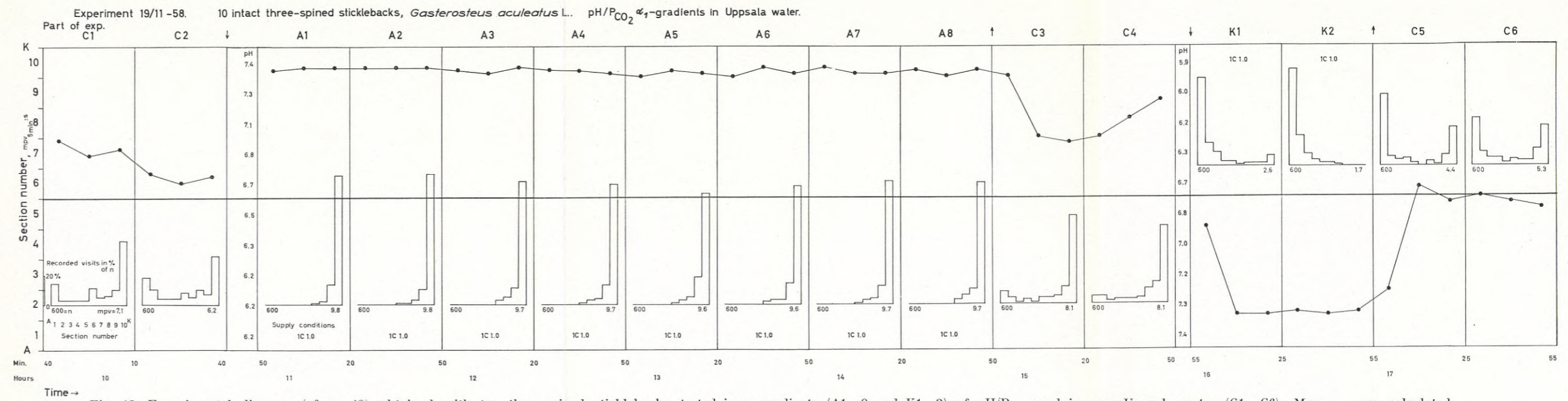
Fig. 13. Experimental diagram (cf. p. 49) obtained with ten three-spined sticklebacks tested in \alpha_1 -gradients (A1—8 and K1—2) of pH/P CO 2 and in pure Uppsala water (C1—C6). mpv_{10min} are calculated.
