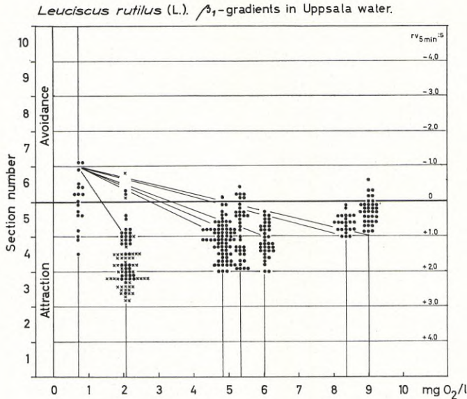
Fig. 26. Rv_{5\text{min}} (dots and crosses) plotted against top concentration of steeper and steeper \beta_1 -gradients of O_2 , which all exhibited the same low concentration level (at about 0.8 mg O_2/l ) on one side of the test yard. Crosses and dots represent fish previously acclimatized to various oxygen regimes (p. 91).
