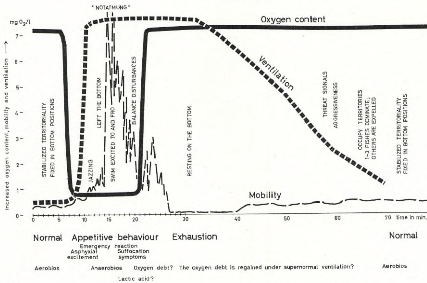
Fig. 27. The essential reactions of salmon parr released at 15 minutes' oxygen depletion all over the test yard. O 2 , ventilation and mobility are visualized as plotted against time. O 2 is analysed (acc. to Winkler) and given as stated by the left-hand vertical scale. Ventilation and mobility are roughly estimated and given according to arbitrary ordinate scales.
