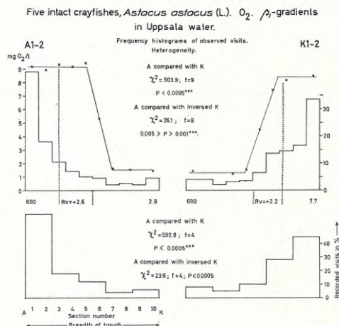
Fig. 28. Preferred sections of crayfish in \beta_1 -gradients of O 2 . Cf. Fig. 25. For the explanations of the statistics see p. 65.
