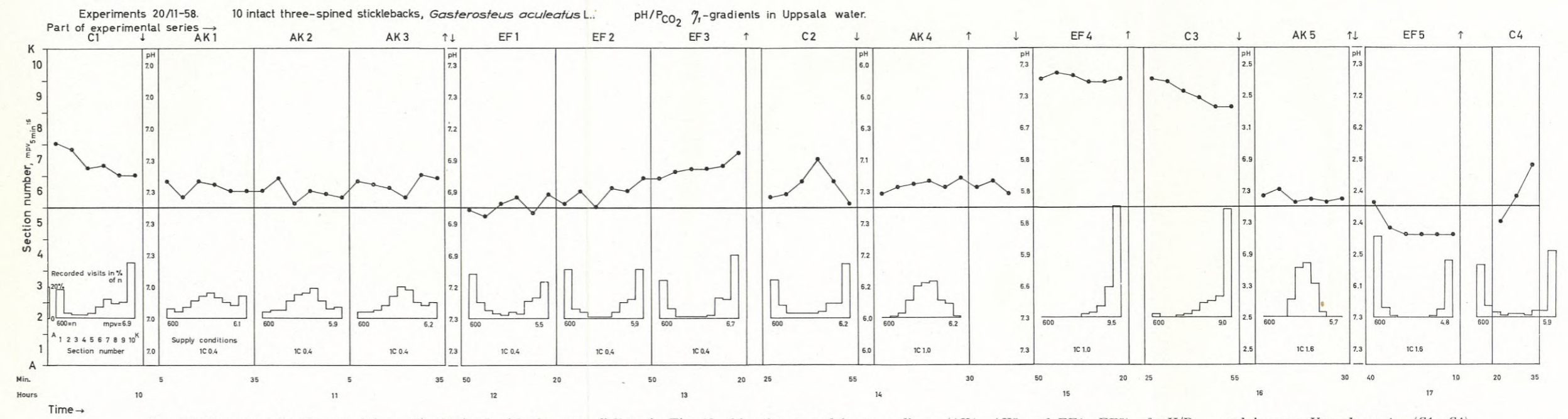
Fig. 14. Experimental diagram (cf. p. 49) obtained with the same fish as in Fig. 13, this time tested in \gamma_1 -gradients (AK1—AK5 and EF1—EF5) of pH/P CO 2 and in pure Uppsala water (C1—C4).
