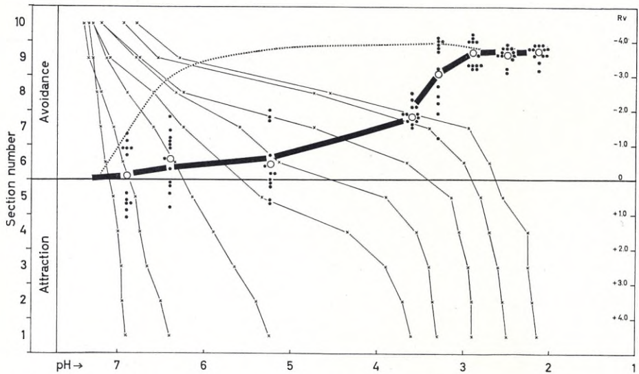
Fig. 30. Reaction diagram (cf. p. 56) showing the reaction curve (heavy one) of salmon parr based on the rv_{5\text{min}} (dots) or rv_{60\text{min}} (circles) obtained in \alpha_1 -gradients of pH/P CO 2 of varying steepness in Hölle water. The curve of short dashes is the reaction curve obtained at approximately the same pH gradients established in Uppsala water (cf. Fig. 29). Cf. also p. 96 and Figs. 33, 36, and 37.
