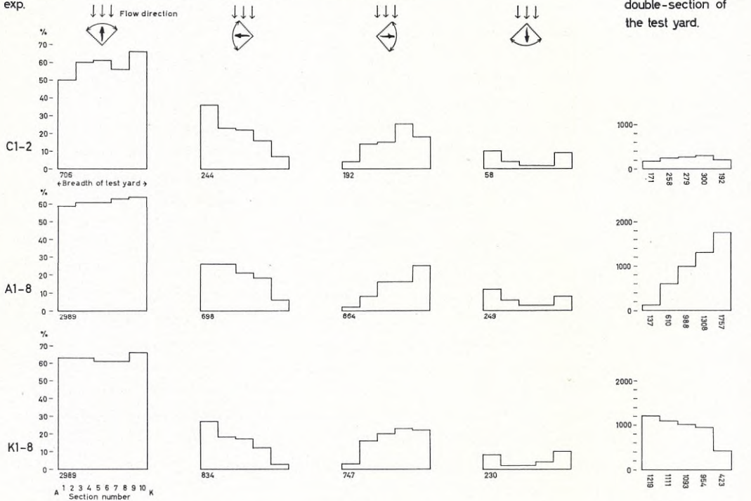
Fig. 21. Rheotactic orientation in different double sections of the test yard during different parts of the experiment of Dec. 18, 1958 (cf. Fig. 11).
