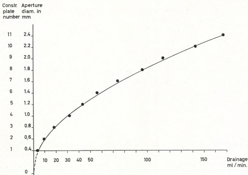
Fig. 5. Aperture diameter of constriction plates in relation to the outflow from Marriotte's flask of tap water at 10°C.
