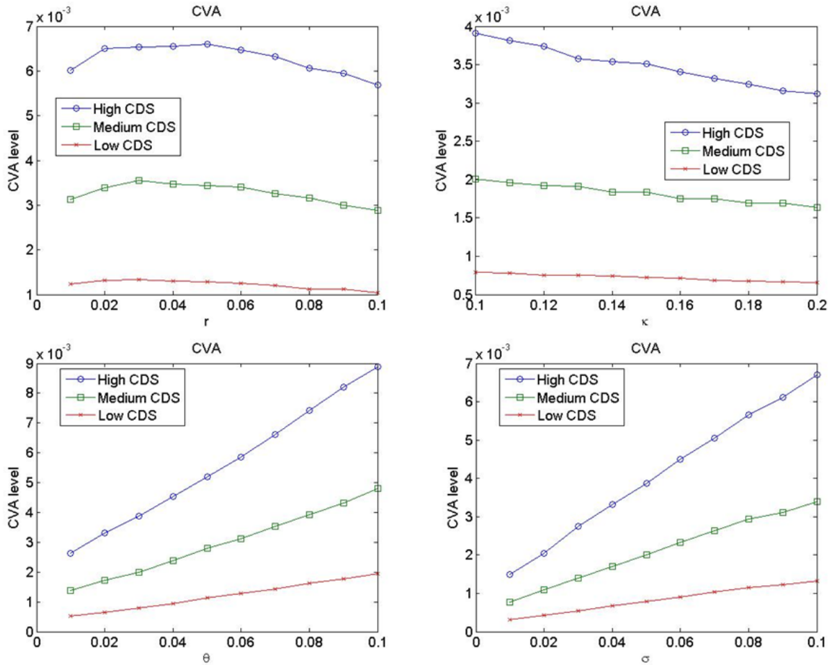
Figure 7.1: The change in CVA as a function of \kappa , \theta , \sigma , r_0 in three CDS scenarios.
