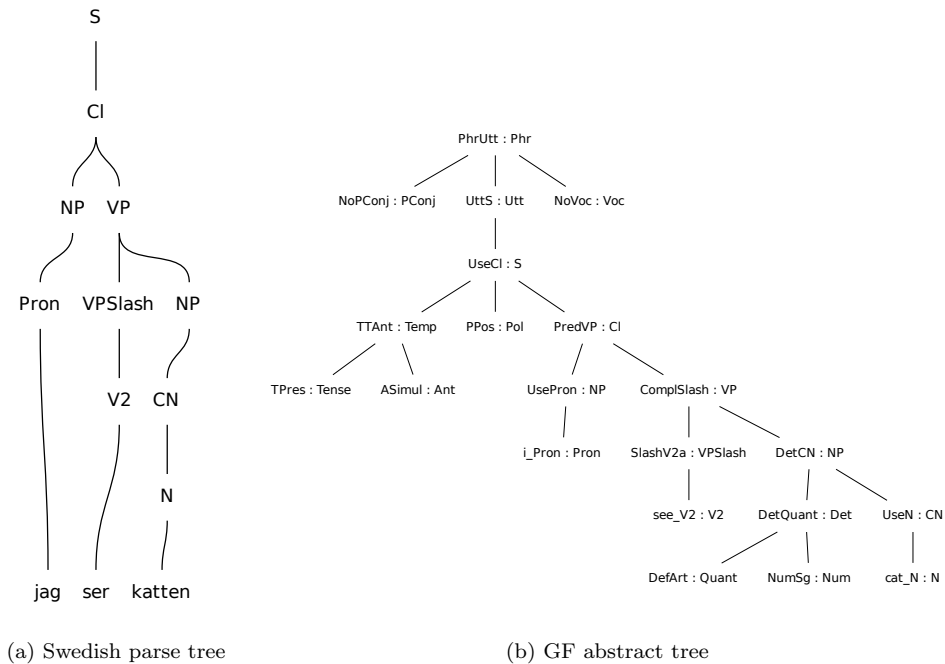
Figure 2.2: Abstract tree and parse tree for the sentence “Jag ser katten”.
