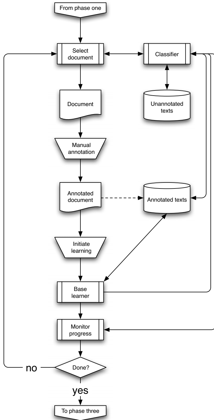
Figure 6.3: Outline of the second phase of the BootMark method.
