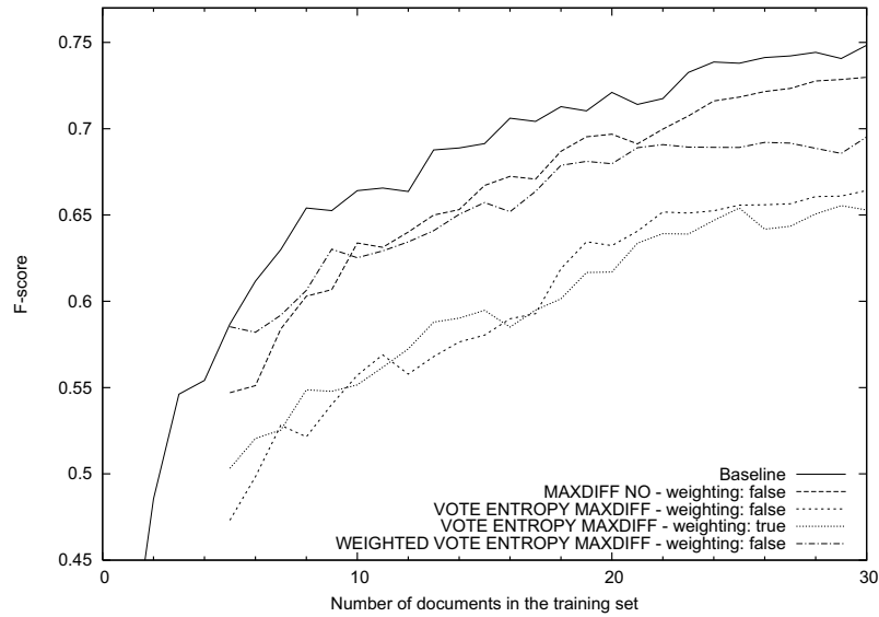
Figure 9.15: Co-testing using the c_0 feature set split with difference-based document selection metrics. The two weighting schemes produce inseparable results for vote entropy maxdiff, hence the inclusion of both vote entropy maxdiff curves.
