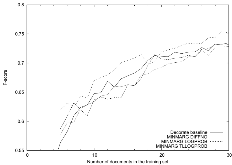
Figure 9.12: ActiveDecorate with margin-based document selection metrics.
