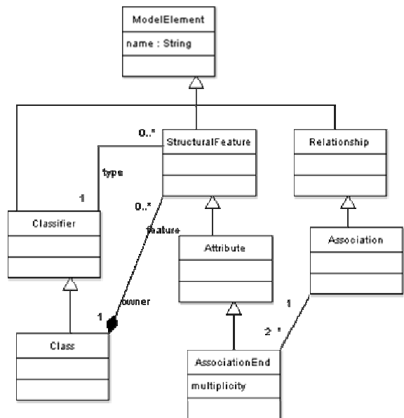
Figure 3 First meta-model candidate
