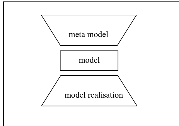
Figure 5 Sand-watch view of MDA relationships
