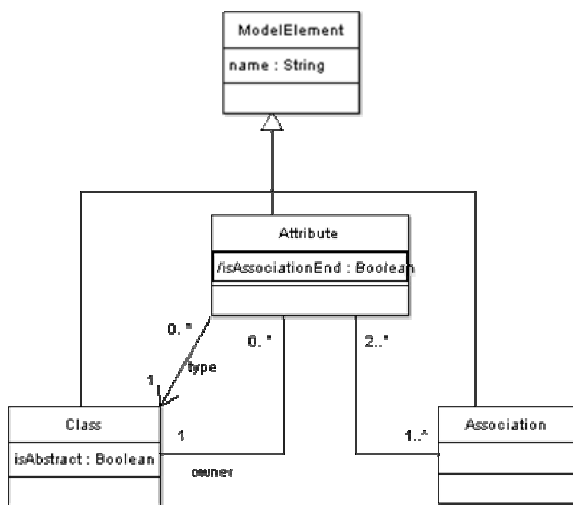
Figure 4 Second meta-model candidate
