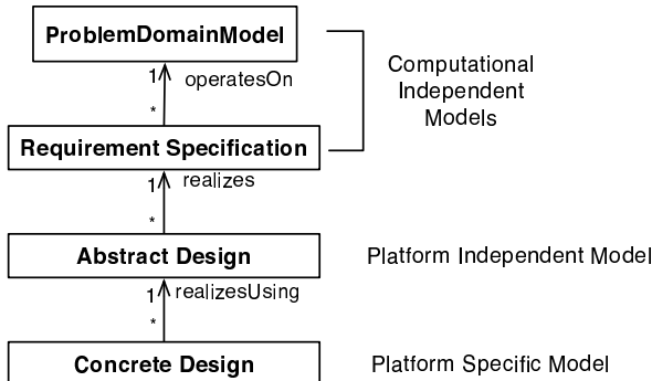
Figure 1. Phases and artifacts.
