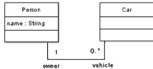
Figure 2 UML model example
